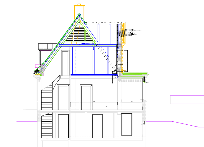
Snit D - D
